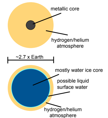
Two possible interior structures of GJ 1214b.
