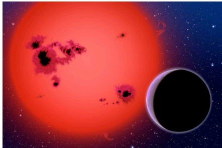
Artist's conception of GJ 1214b - a 'Super Earth' orbiting a star ~40 light-years away. The planet orbits at a distance of only ~15 stellar radii. Image from David Aguilar.
