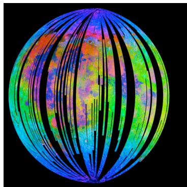
This false-color map created from data taken by NASA's Moon Mineralogy Mapper (M3) on Chandrayaan is shaded blue where trace amounts of water (H 2 O) and hydroxyl (OH) lie in the top few mm of the surface.
