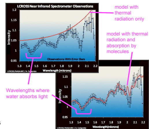
An infrared spectrum measured by LCROSS (black data points) compared to models (red line)
